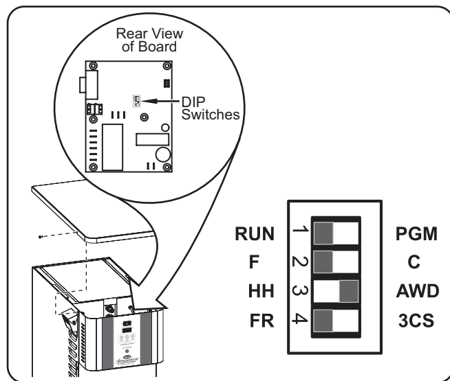
Dipswitch Controls
