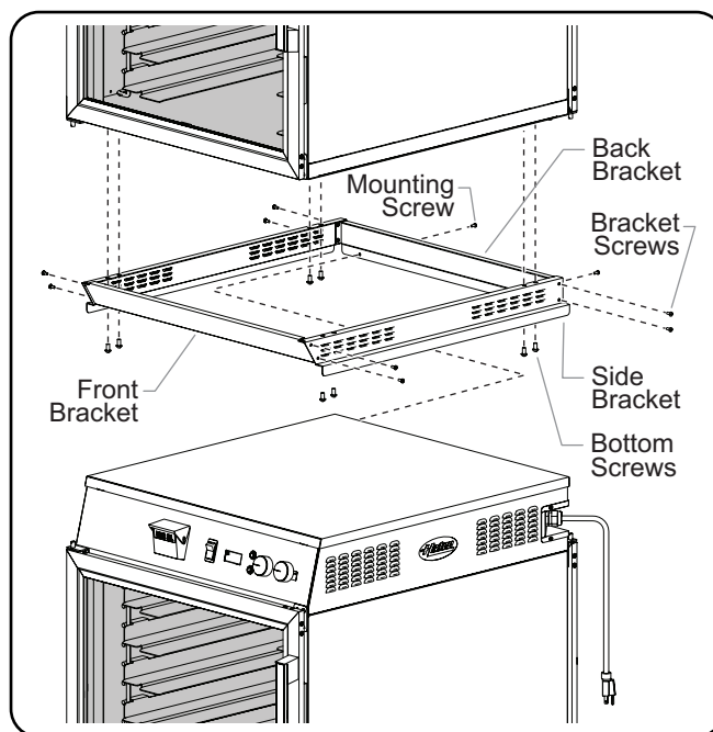
Stacking two units
