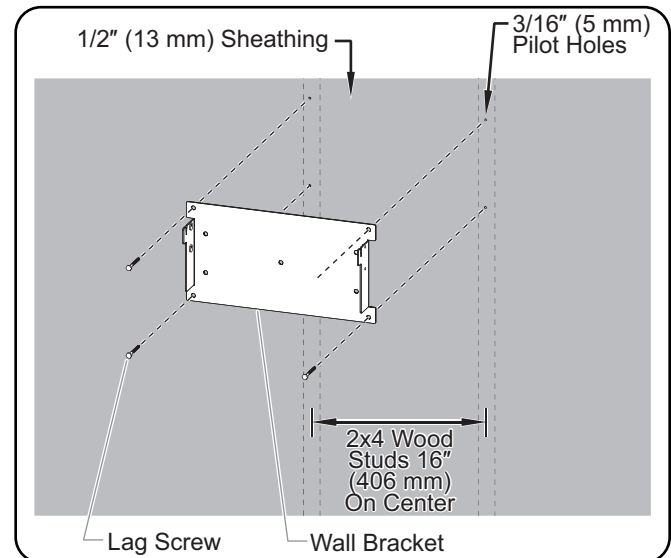
Attaching the Wall Bracket
