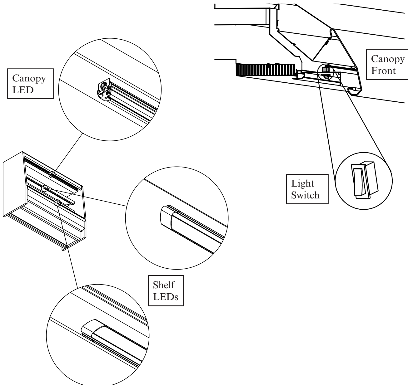
(EcoShine LED Bars Shown)
