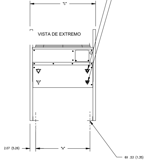
END VIEW
