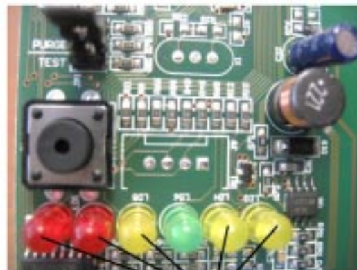
ALL STEADY CALIBRATION OF PC BOARD & OPTICAL ICE LEVEL CONTROL
