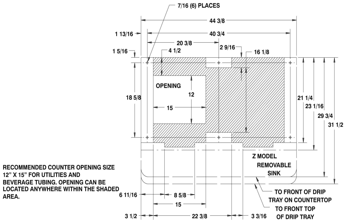
Figure 8 Mounting Template (BC models)
