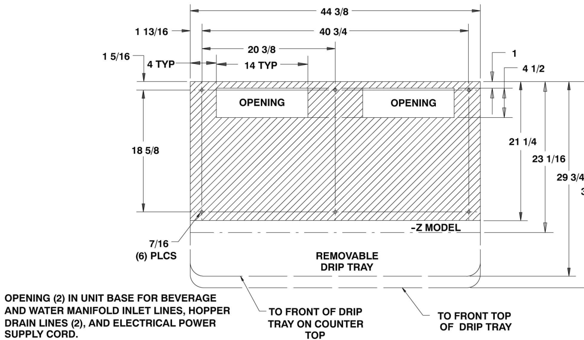
Figure 7 Mounting Template (Ice only- B models)
