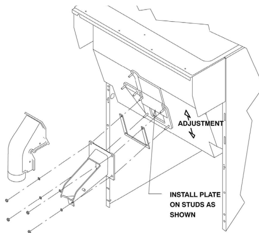
Figure 1 Gate Restrictor Plate
