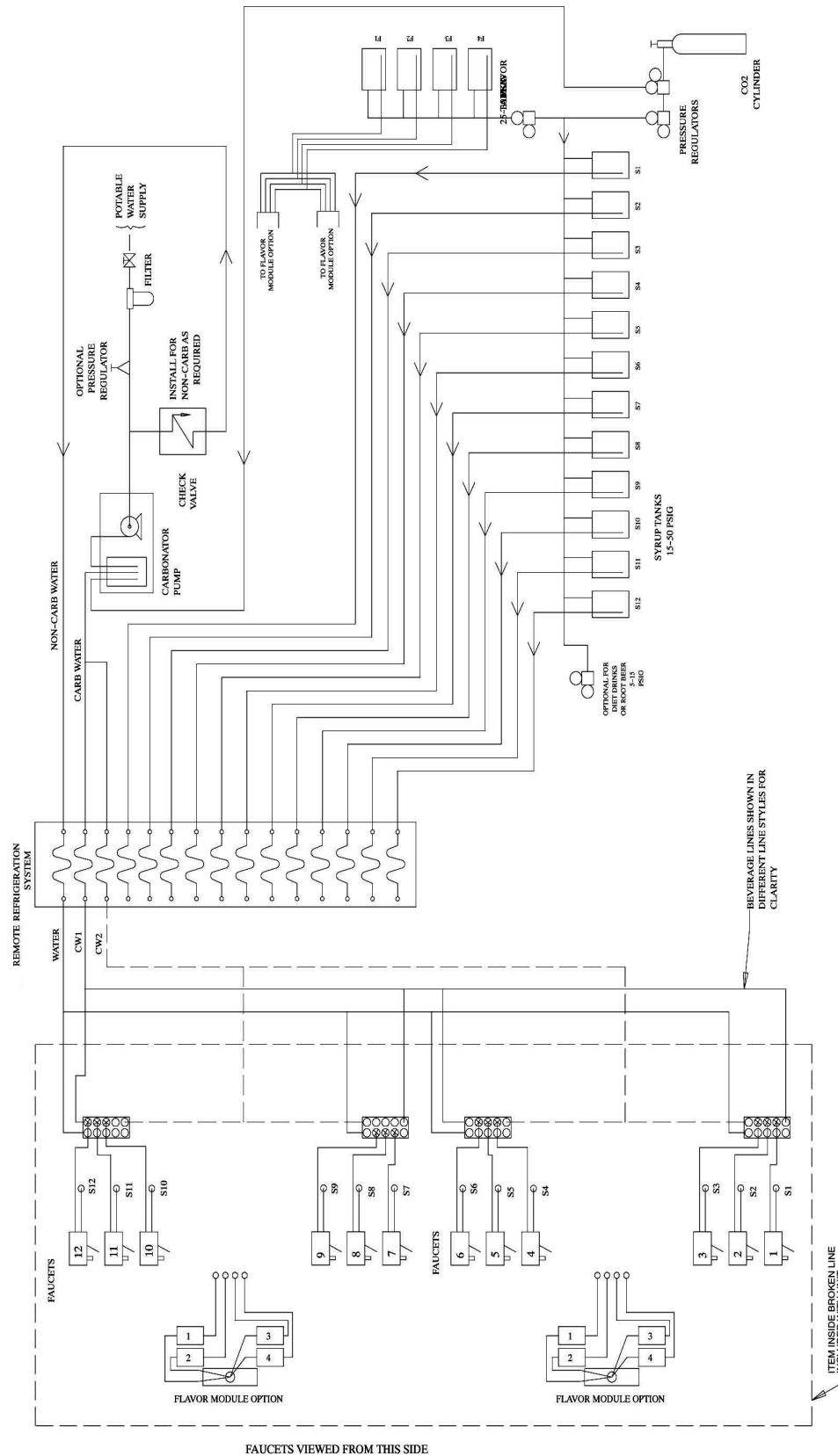
Figure 4 Flow Diagram (B Models with Twelve Beverage Faucets)
