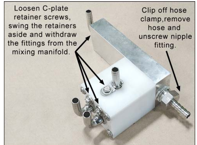
Figure 6-4 - Mixing Manifold Hose Fittings Removal
