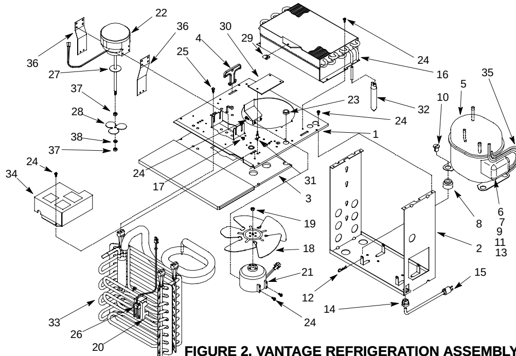
FIGURE 2. VANTAGE REFRIGERATION ASSEMBLY
