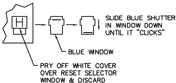
Motor Overload Relay
