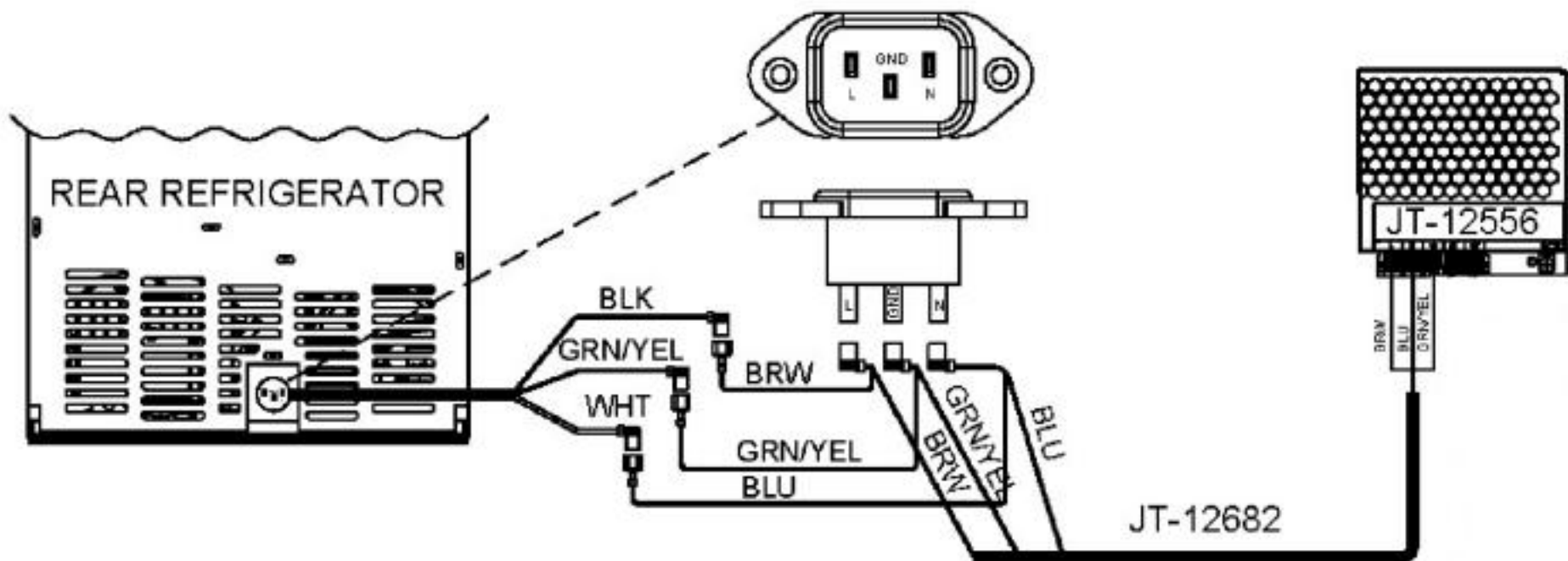
Figure 1a: Power Supply Harness Diagram.
