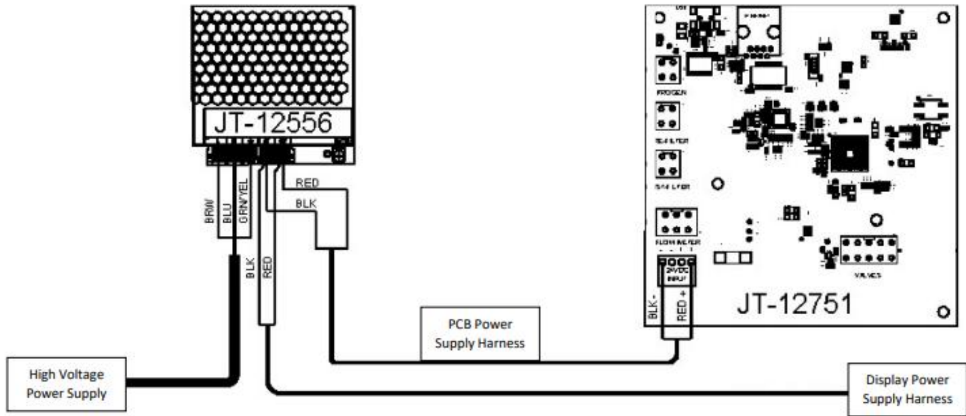
Figure 4: Power Supply Cables Schematic.
