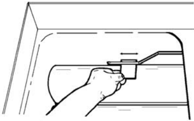
Thermostat Bulb Positioning 18" & up Fryer Gas
