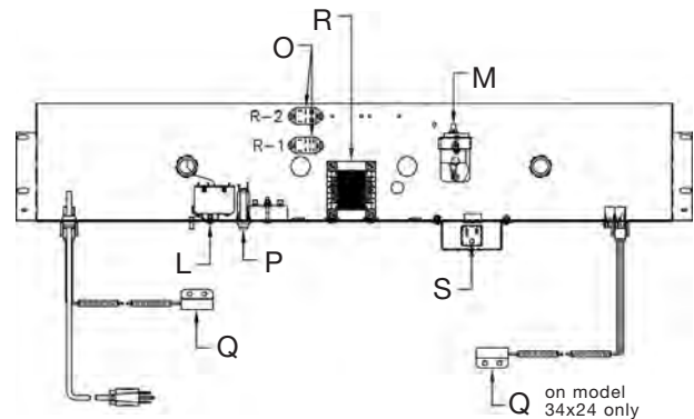
Back Panel - Rear Drain Unit
