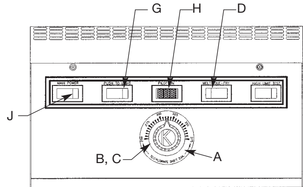
Control Panel Front
