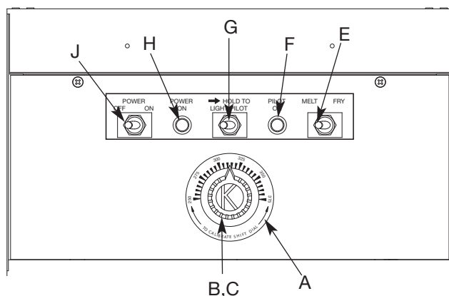
Control Panel Front
