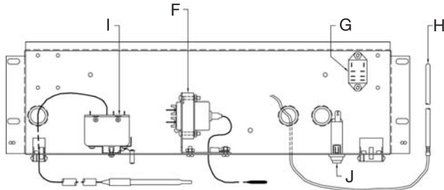
Back Panel - Rear Drain Unit
