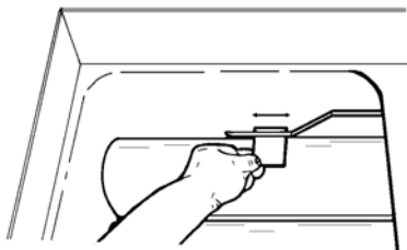
Thermostat Bulb Positioning 10x11, 18 & larger Fryer Gas
