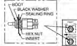
DETAIL - SURROUND ASSEMBLY
