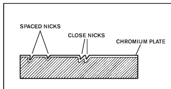
Figure 3-3 Surface Damage
