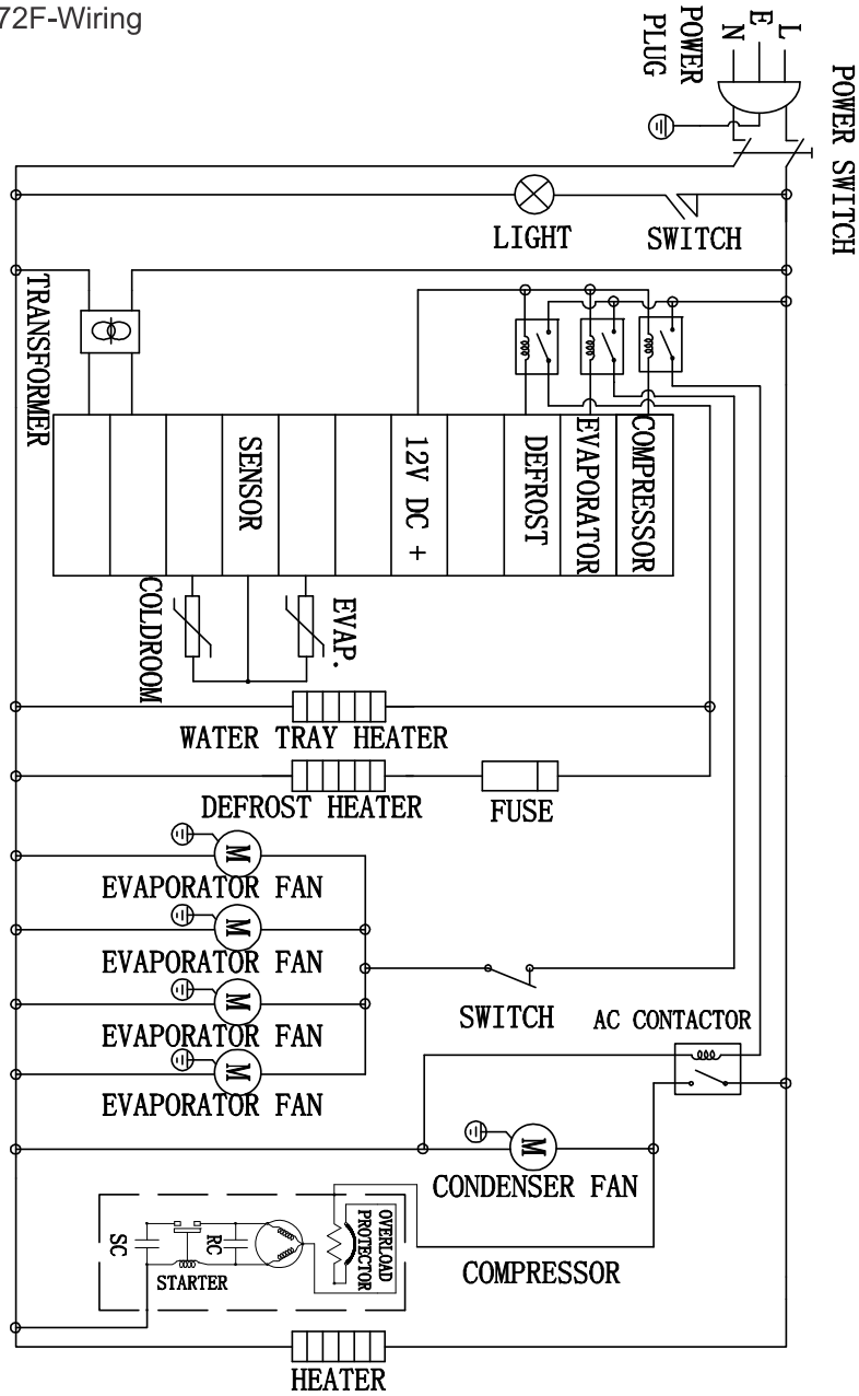
CIRCUIT DIAGRAM
