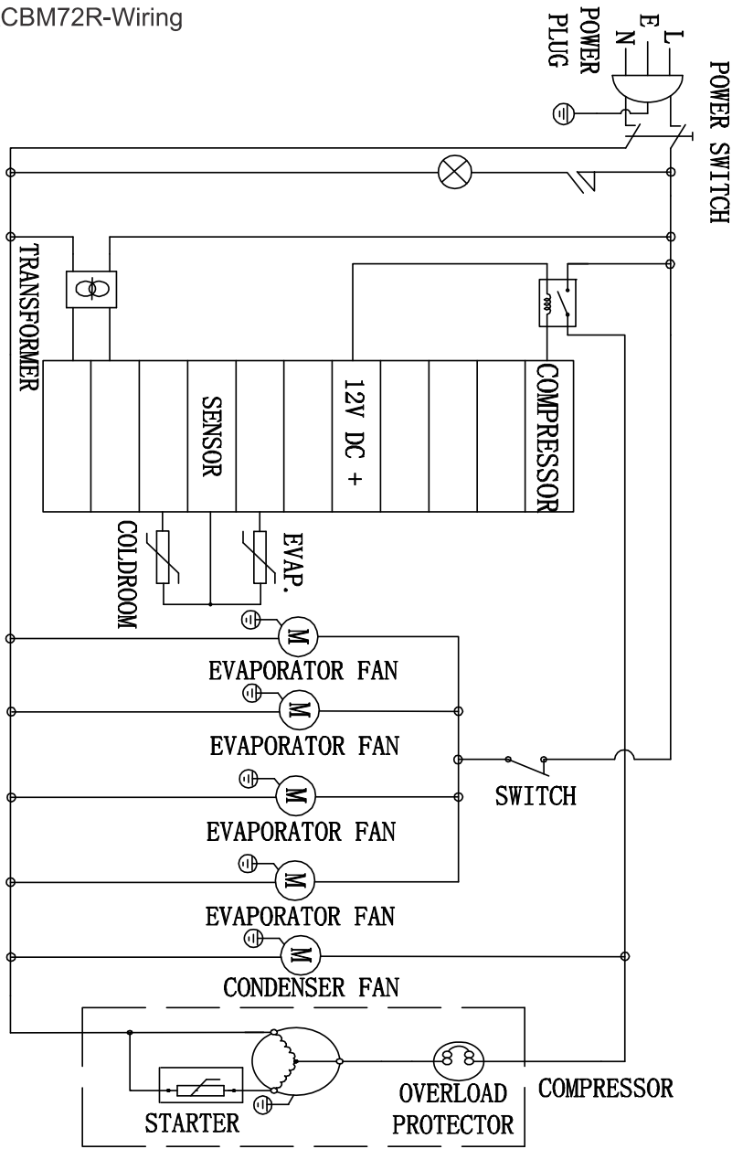
CIRCUIT DIAGRAM
