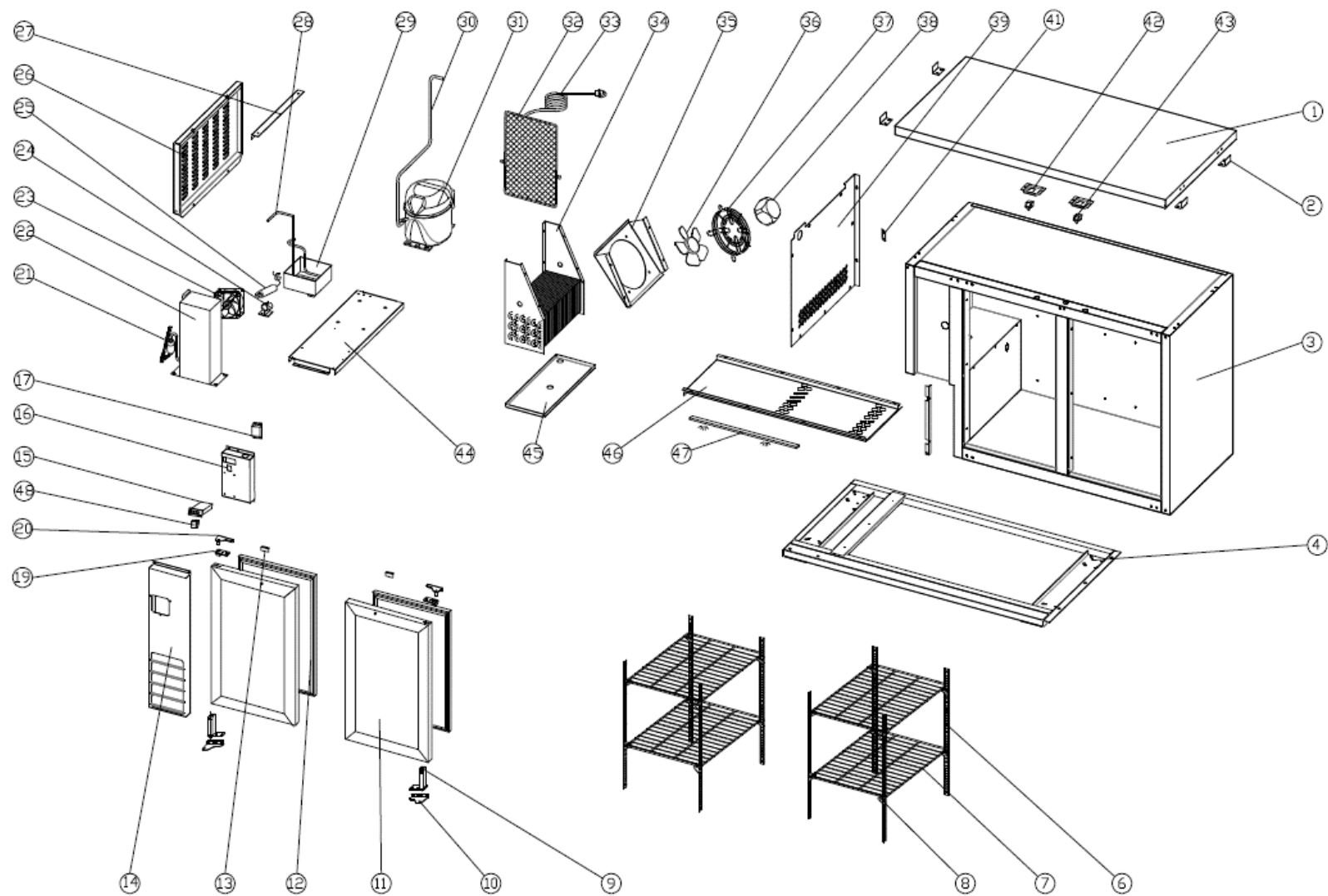
EXPLODE DRAWING OF KCHBB60G
