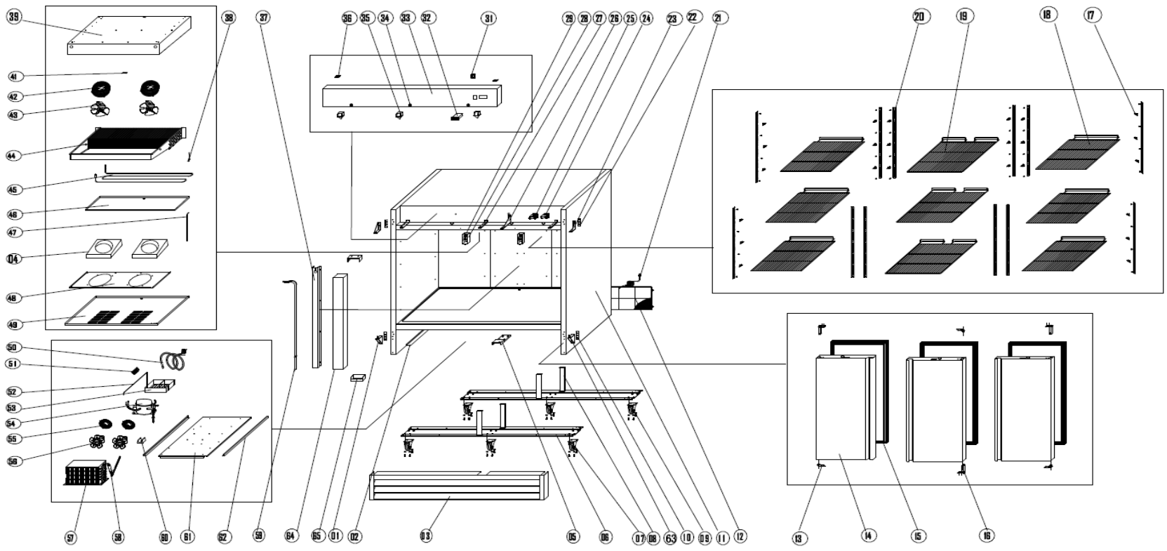
EXPLODE OF KCHRI81R3DF
