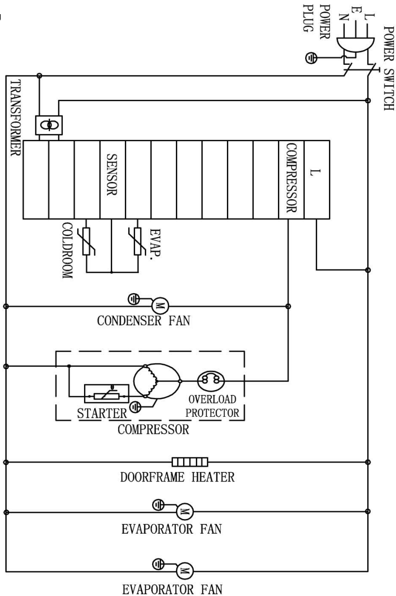
CIRCUIT DIAGRAM
