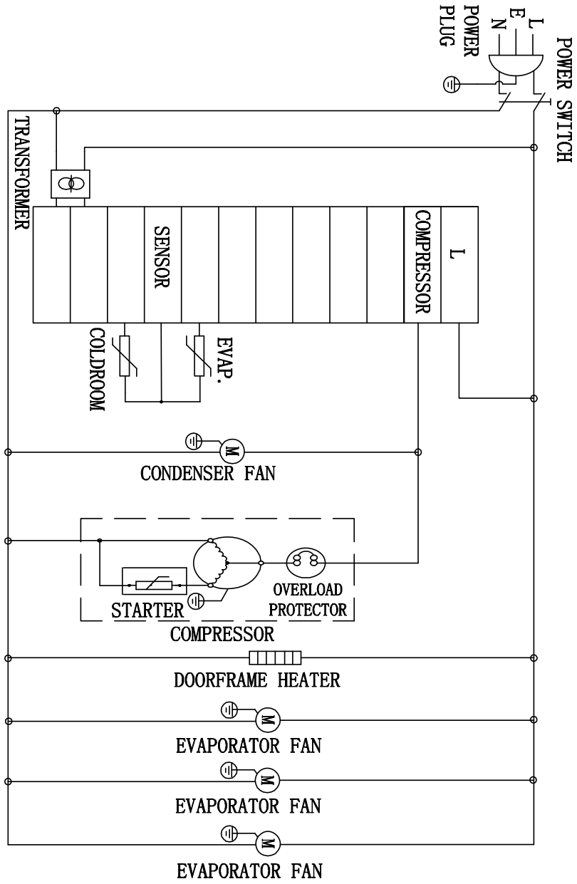
CIRCUIT DIAGRAM
