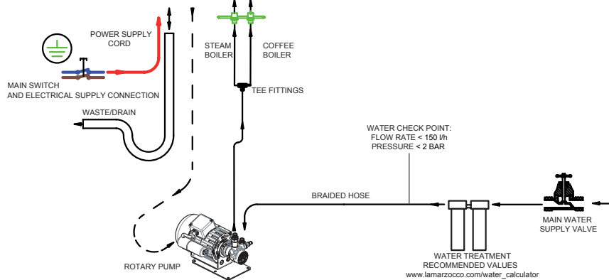
Fig. 4 - Installation guide - type 1
