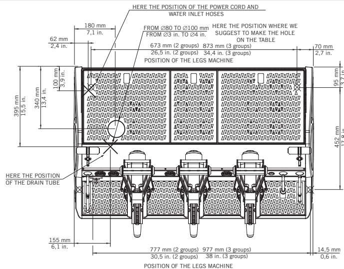
Fig. 3 - Installation guide
