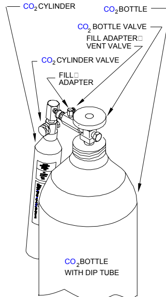
CO 2 Filling Instructions Figure 8
