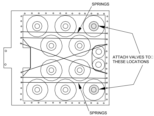
Bottle Hold Down Springs and Bottle Placement
