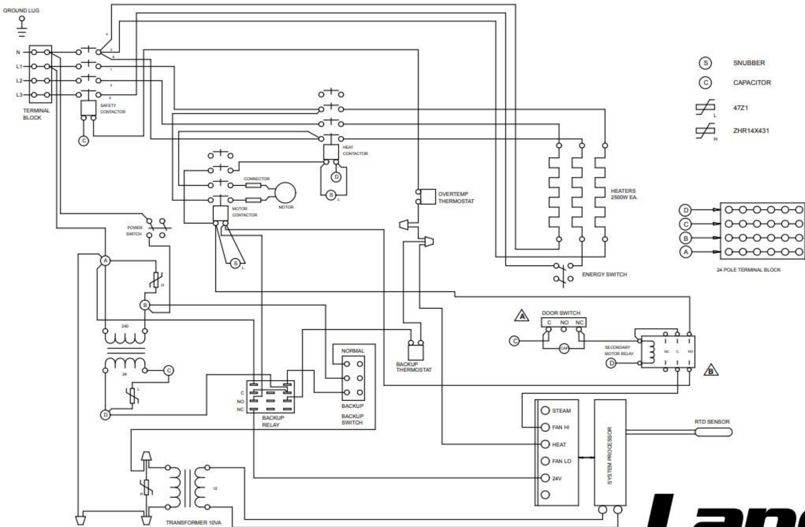
MODELS: ECOH-2/4CECN Electric Half Size Convection Oven
