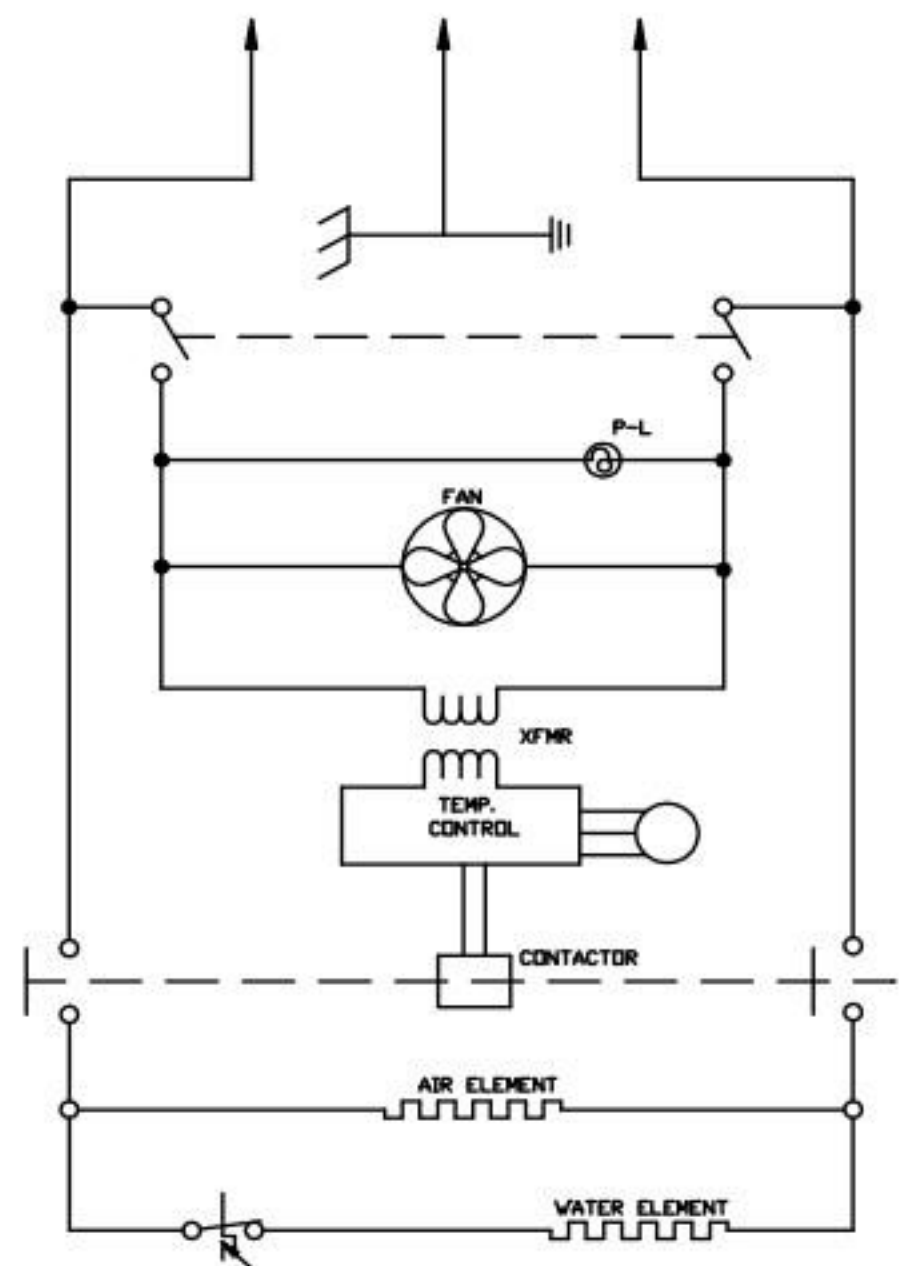
SCHEMATIC DIAGRAM
