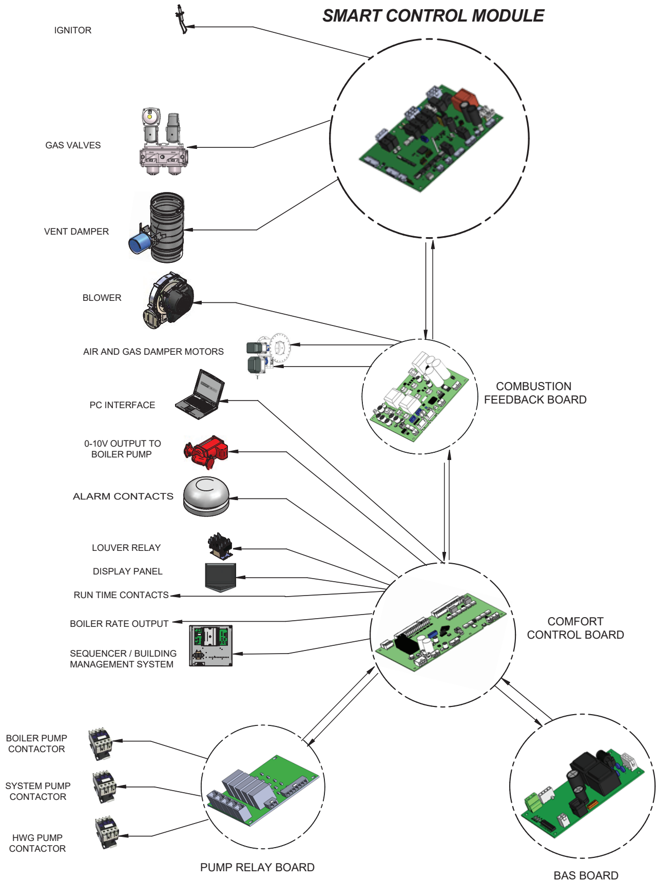
Figure 6-3A Crest - Control Outputs
