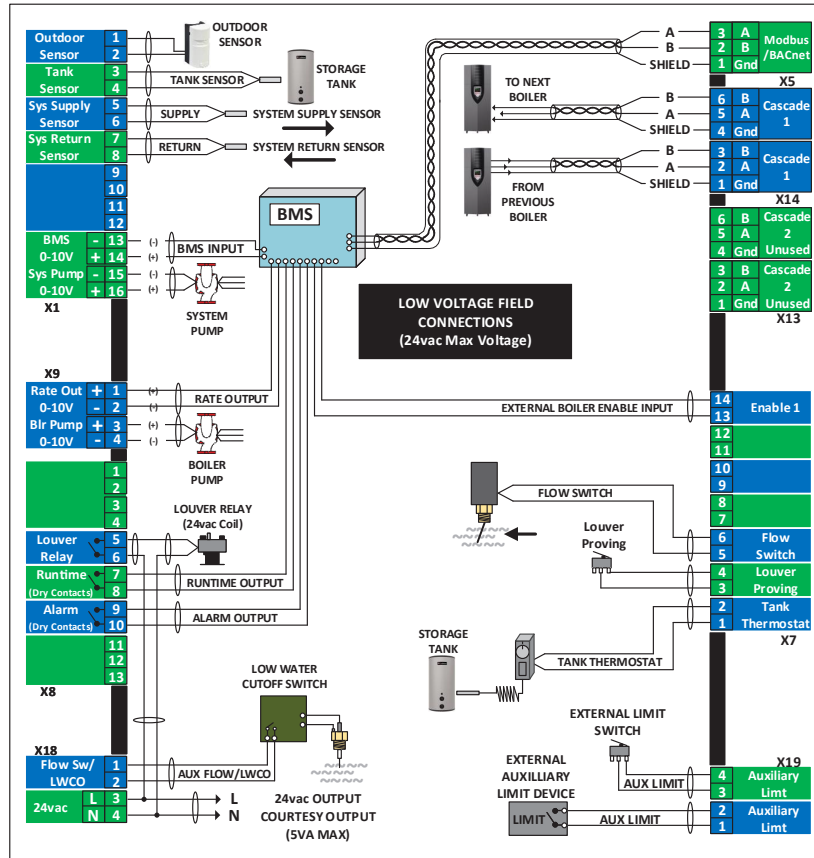
Figure 6-1B Hellcat- Low Voltage Terminal Strip Connections
