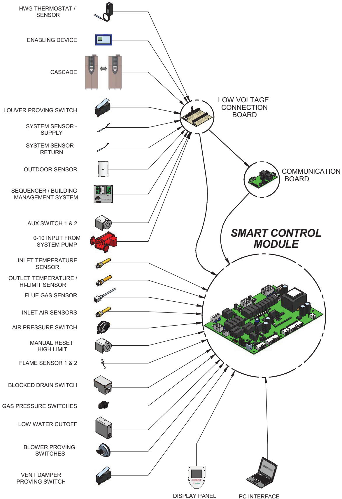
Figure 6-2B Hellcat - Control Inputs
