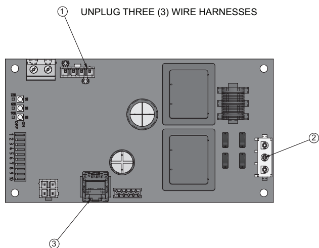
Figure 8-1 _Communication Board
