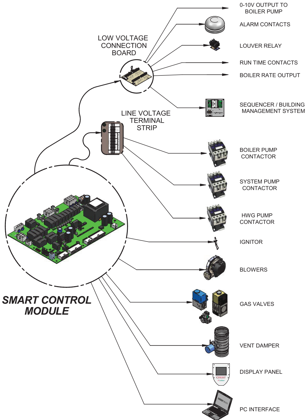
Figure 6-3B Hellcat - Control Outputs
