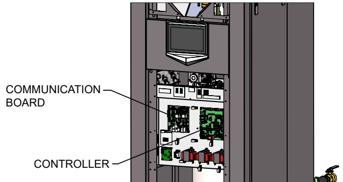
Figure 6-4B Hellcat - Control Location
