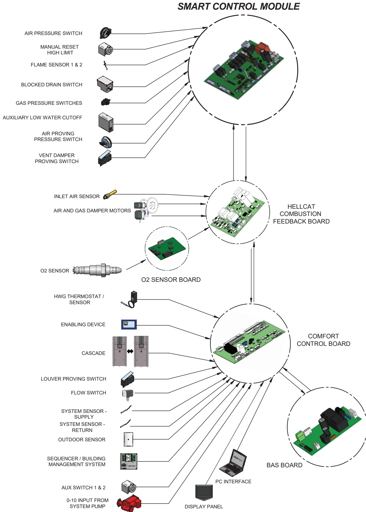
Figure 6-2A Crest - Control Inputs
