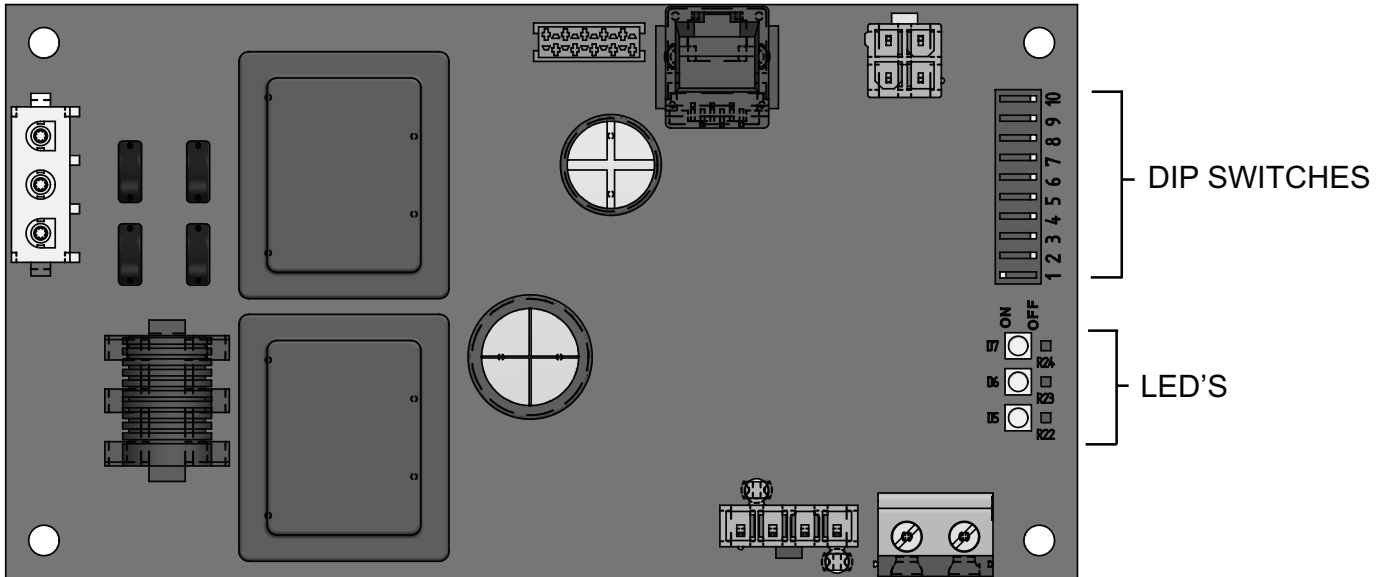
Figure 2-1_Communication Board
