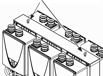
Figure 3: Lifting Eyebolts
