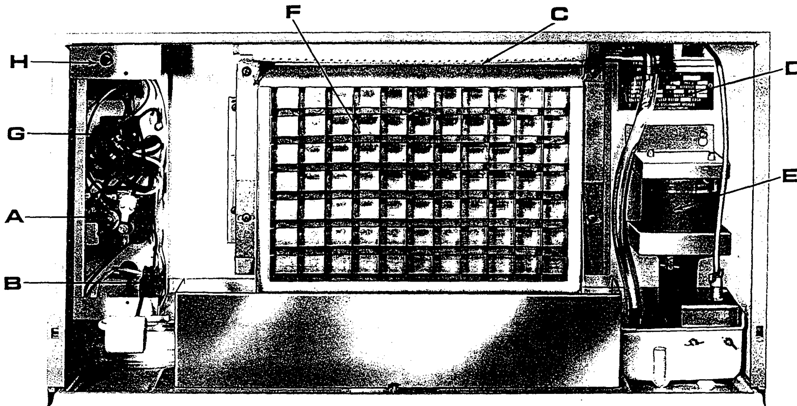
FIG. 2 FRONT WITH SPLASH CURTAIN REMOVED
