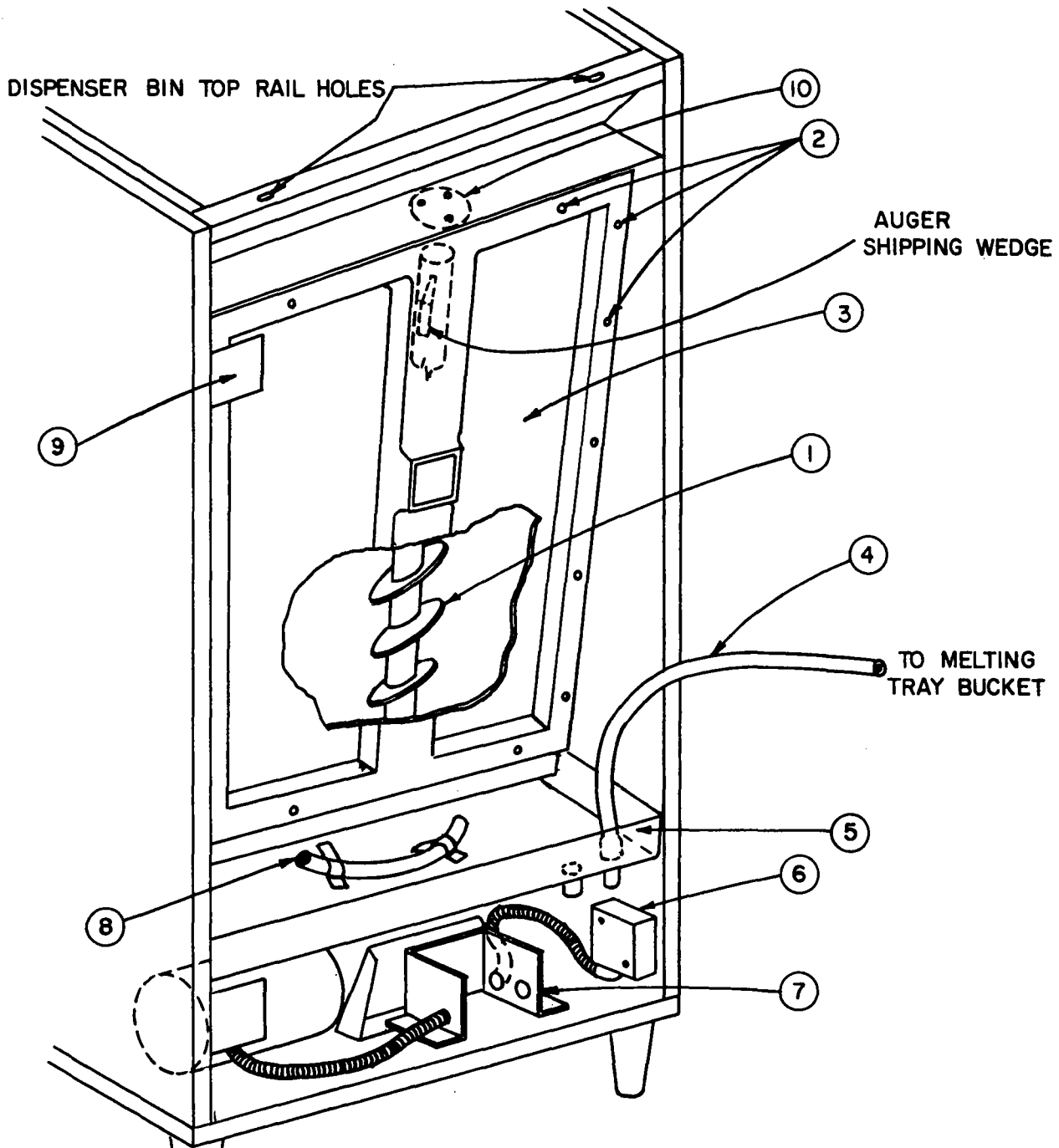
FIG. 6 INTERNAL VIEW OF DISPENSING BIN
