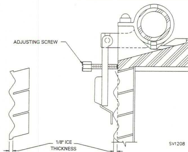
Figure 7. ICE THICKNESS CHECK
