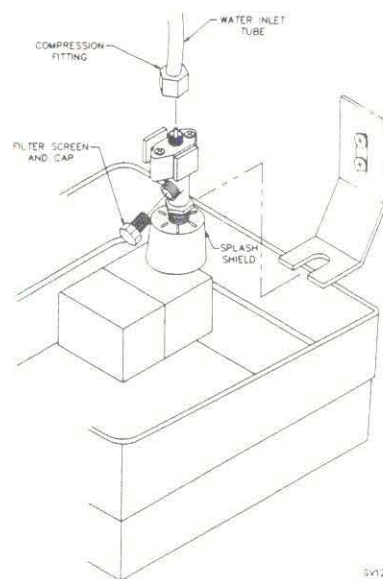
Figure 15. FLOAT VALVE REMOVAL
