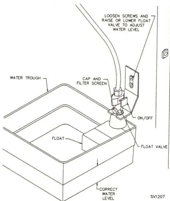
Figure 6. WATER LEVEL CHECK
