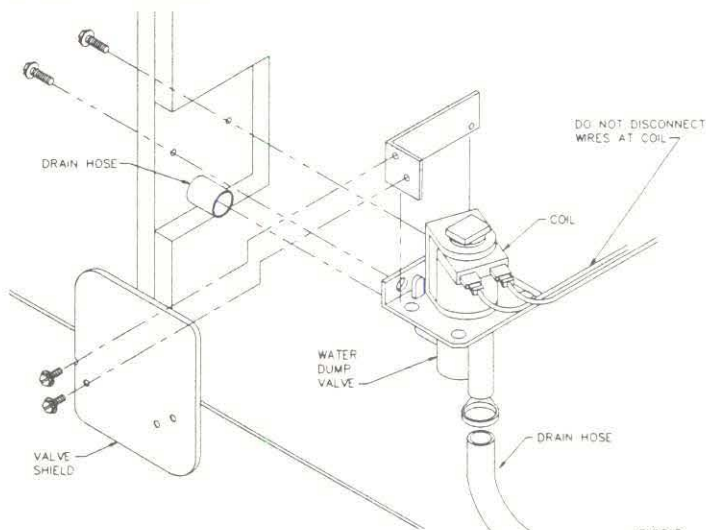
Figure 11. DUMP VALVE REMOVAL
