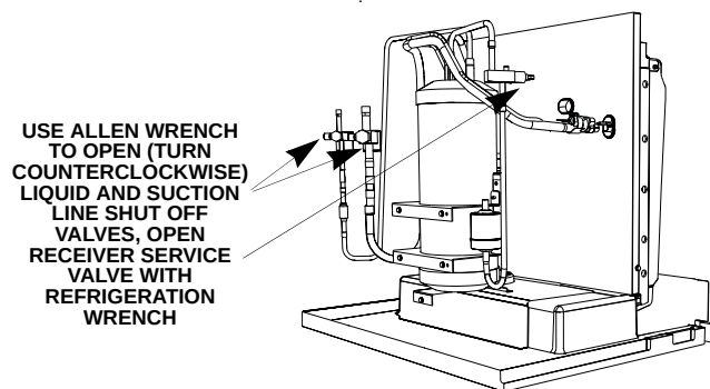
30" Single Evaporator Models
