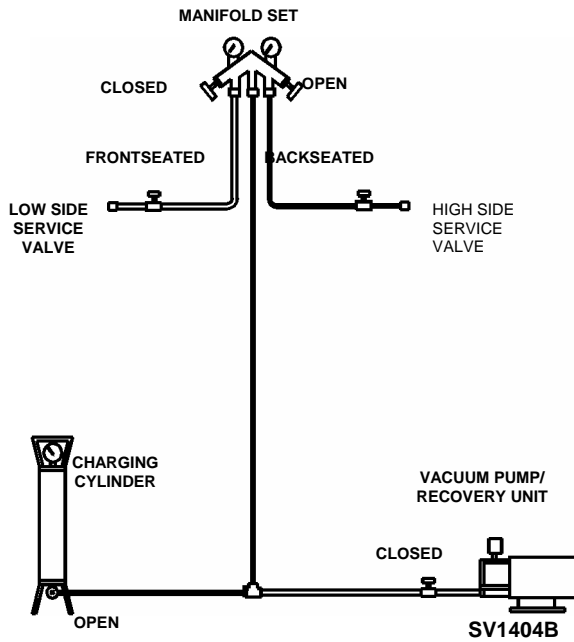
Charging Connections
