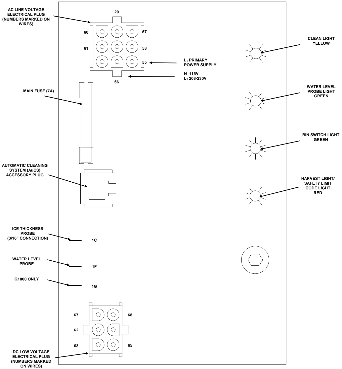
Control Board
