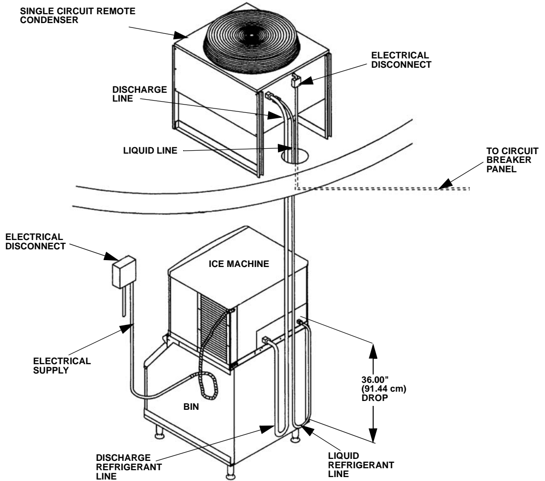
Typical Single Circuit Traditional Remote Condenser Installation
