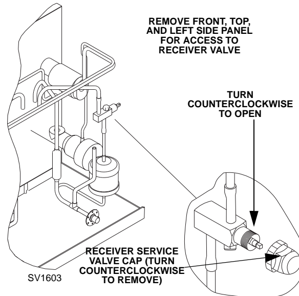
Backseating the Receiver Service Valve
