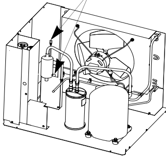
ALTERNATE CONNECTIONS AT CONDENSING UNIT SCHRADER VALVES
