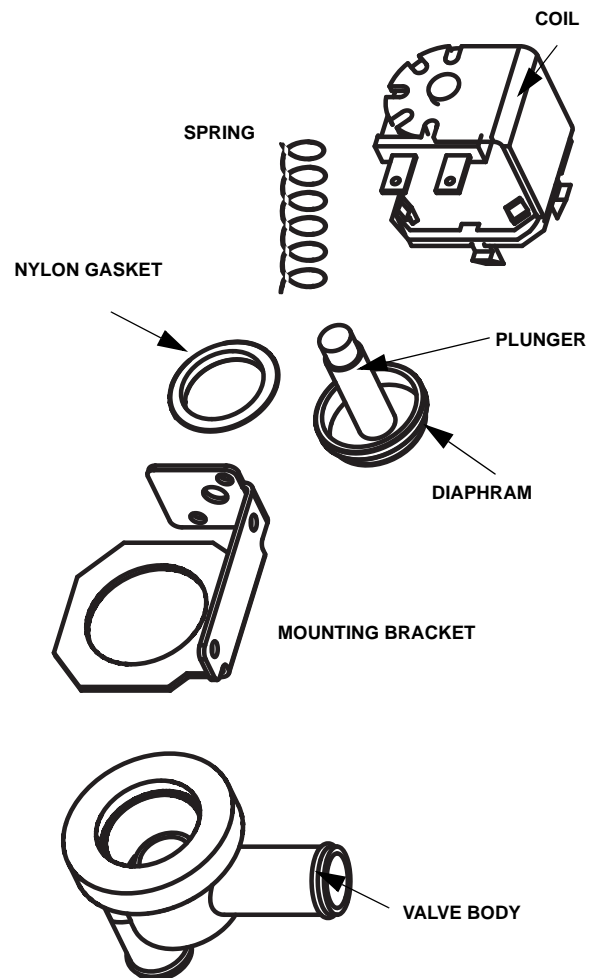
Dump Valve Disassembly
