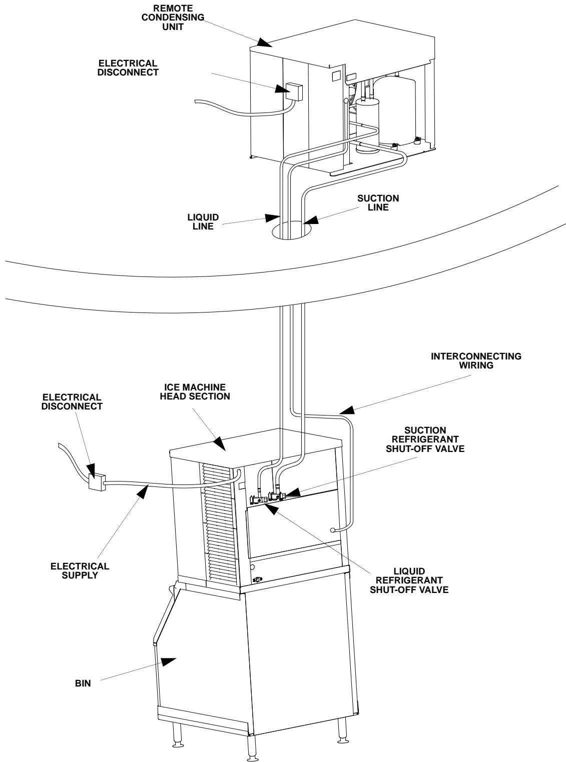
Typical QuietQube System Installation
