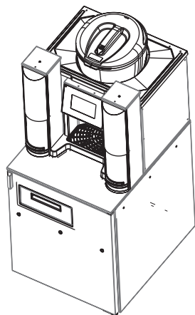
Dual Blend Chamber without Cup Dispenser
