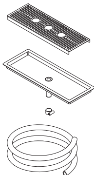
Flush Mount Drain — 020001388
