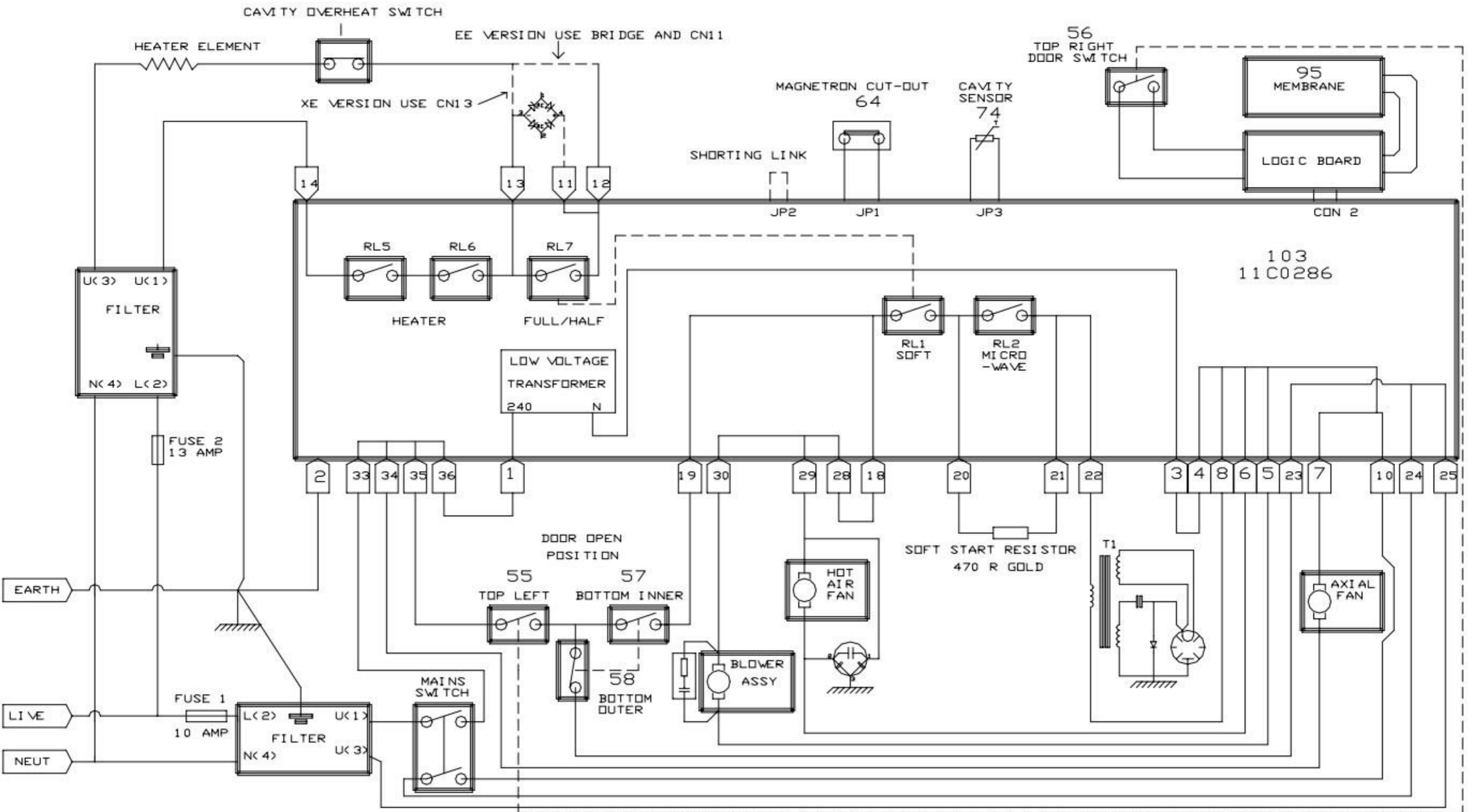
WIRING DIAGRAM - MICROWAIRE SERIES 5 EE (13A) AND XE (30A)
