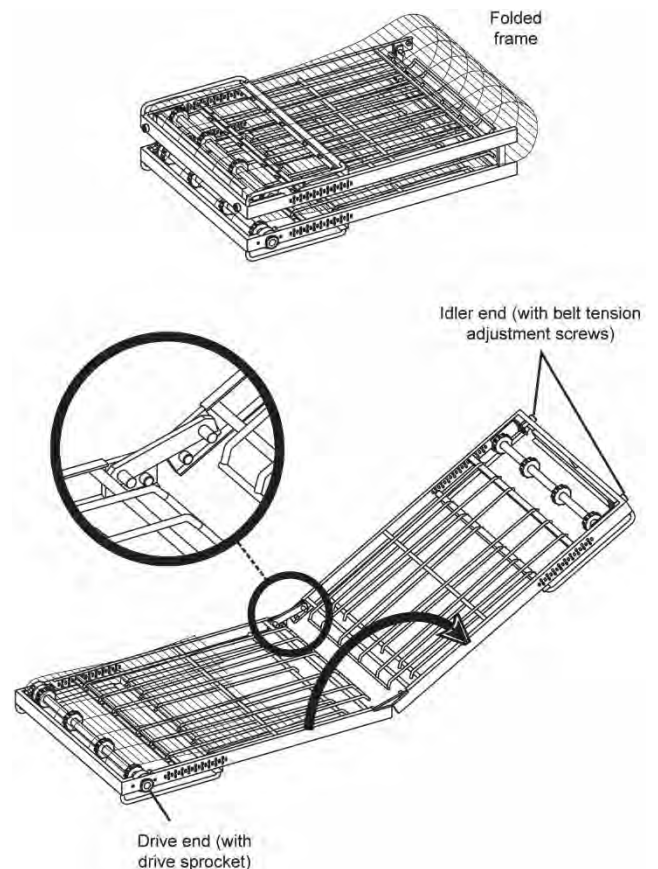
Figure 14. Conveyor Installation
