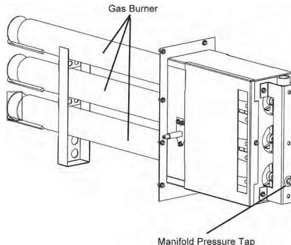
Figure 21. Gas Burner Assembly
