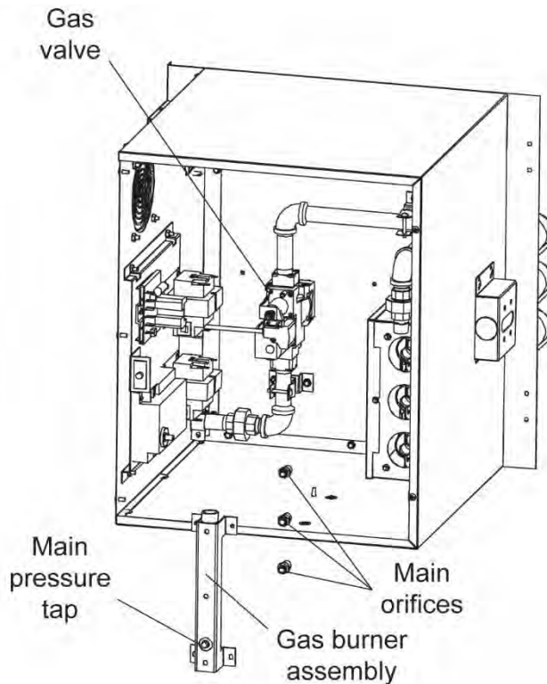
Figure 22. Burner Assembly
