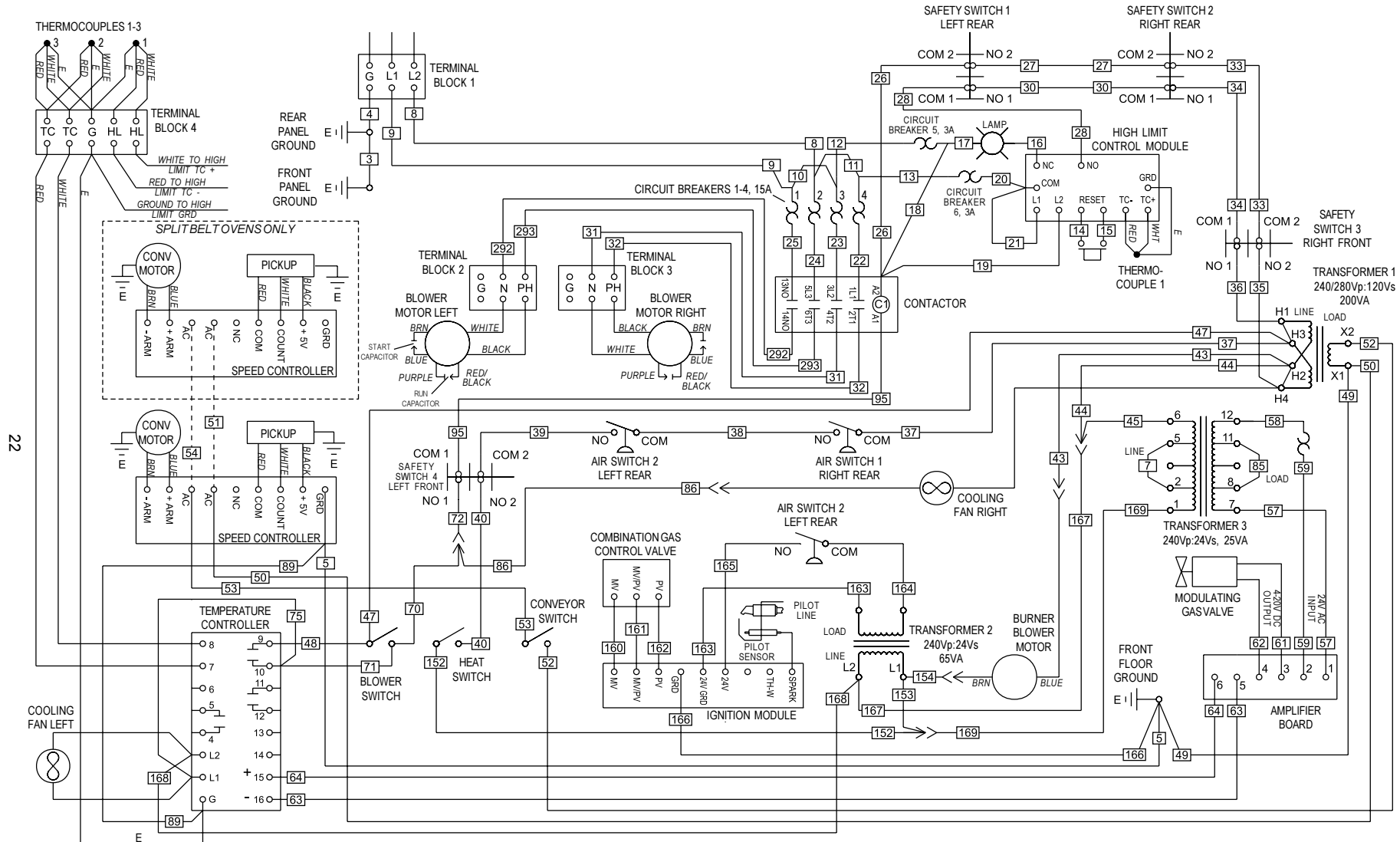
Fig. 5-1 Wiring diagram, PS555G or PS570G Gas Oven, 208/240V, 50/60Hz, 1 Ph
