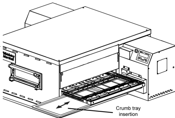
Figure 2-16. Crumb Trays
