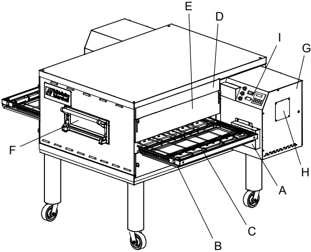
Figure 1-1. Oven Components
