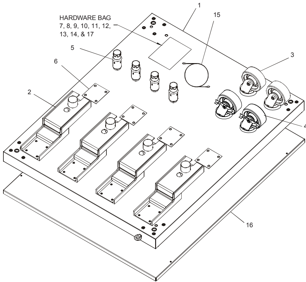
Figure 2-4. Model PS745 Triple Oven Option Base with Outriggers and Top
