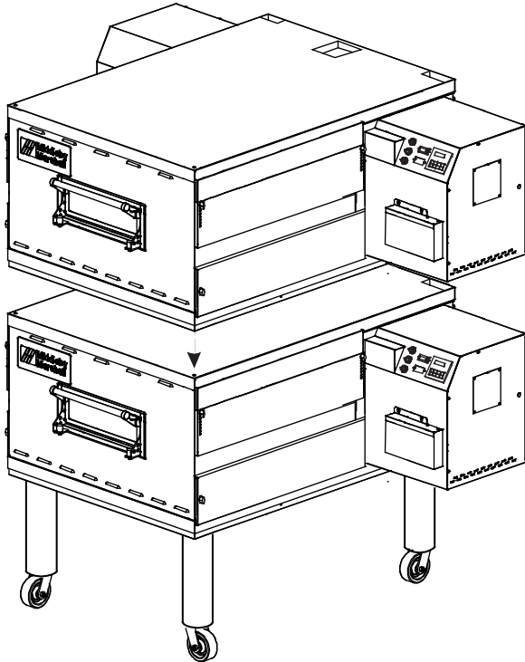
Figure 2-9. Stacking
