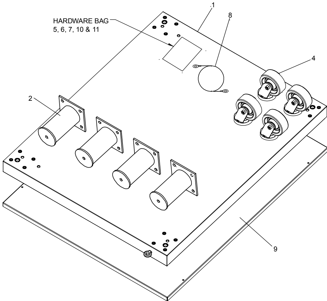
Figure 2-3. Model PS745 Double Oven Option Base with Legs and Top
