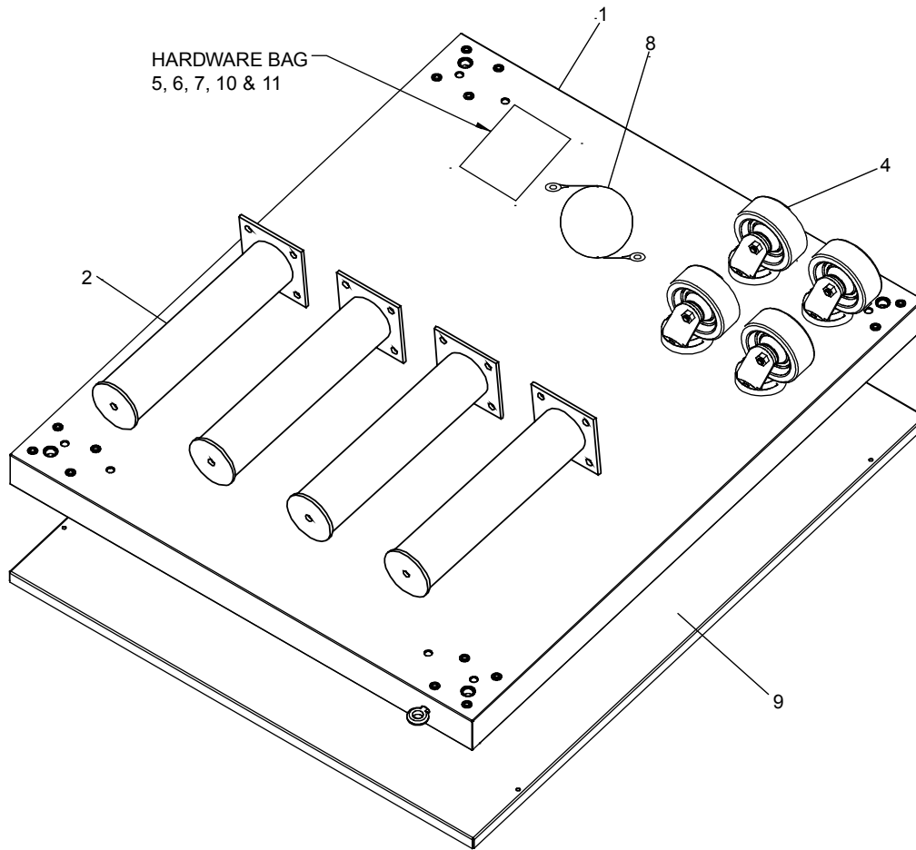
Figure 2-2. Model PS745 Single Oven Option Base with Legs and Top
