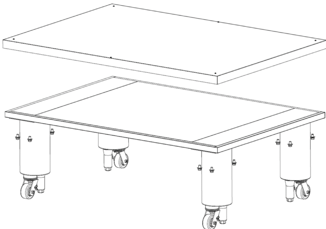
View of X70G/X55G OVEN BASE/TOP KIT with 15" LEGS
