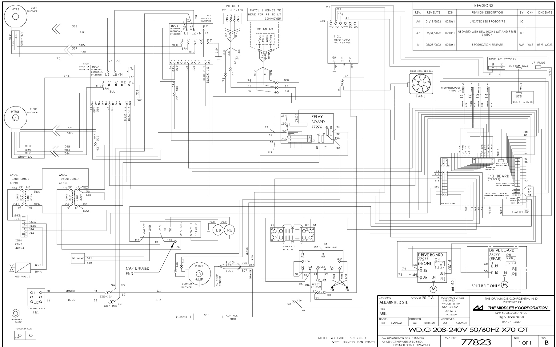
MIDDLEBY MARSHALL X70G WIRING DIAGRAM G208-240 volt 50/60 Hz, 1 Phase
