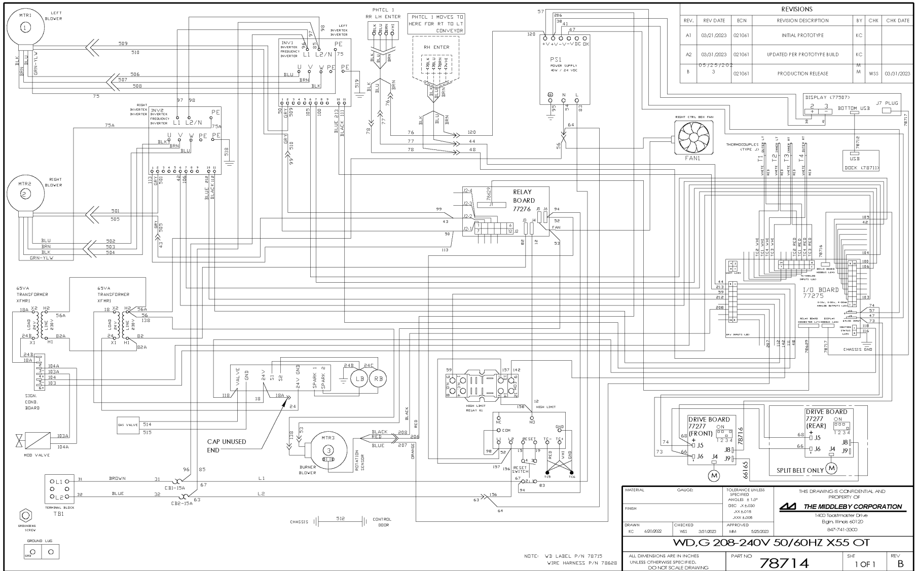
MIDDLEBY MARSHALL X55G/x55GWB WIRING DIAGRAM G208-240 volt 50/60 Hz, 1 Phase
