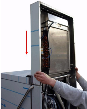
13. Fit the hood/cover for the heat exchanger.
