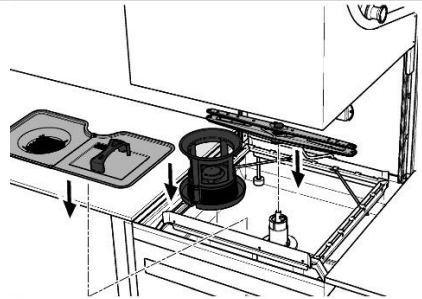
5. Insert the filter, the tank cover sieve and the wash systems.
