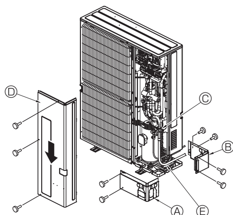
A Front piping cover B Piping cover C Stop valve D Service panel E Bend radius : 100 mm - 150 mm (3-15/16" – 5-7/8")
