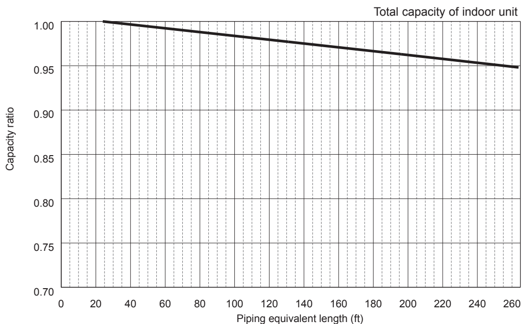
Figure 17 PUMY-P60NKMU2(-BS) <Heating>
