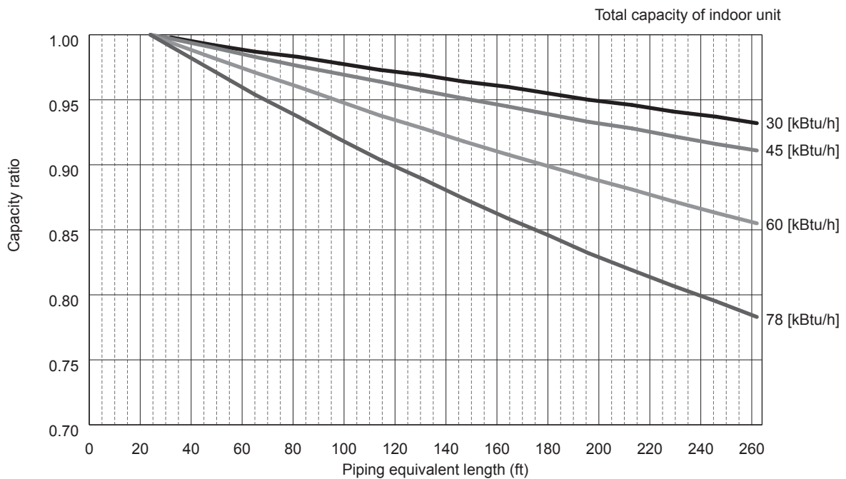
Figure 16 PUMY-P60NKMU2(-BS) <Cooling>
