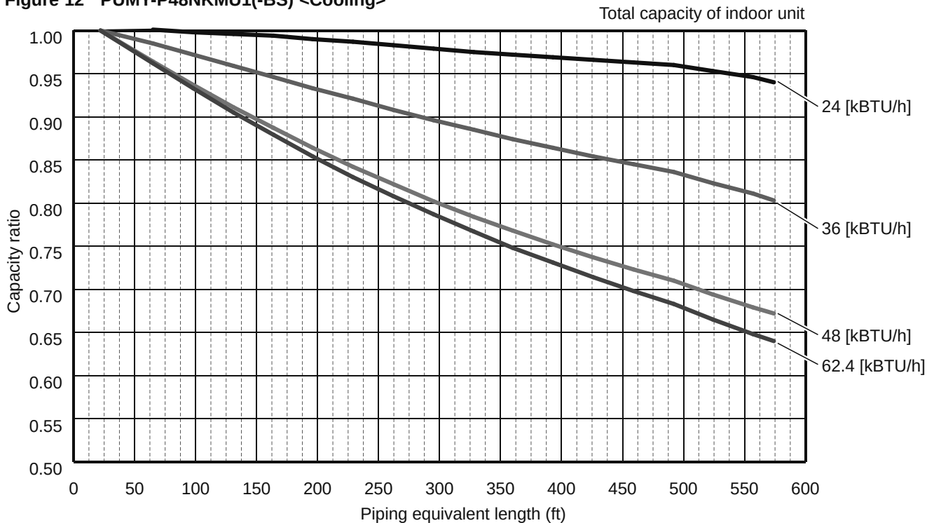
Figure 12 PUMY-P48NKMU1(-BS) <Cooling>
