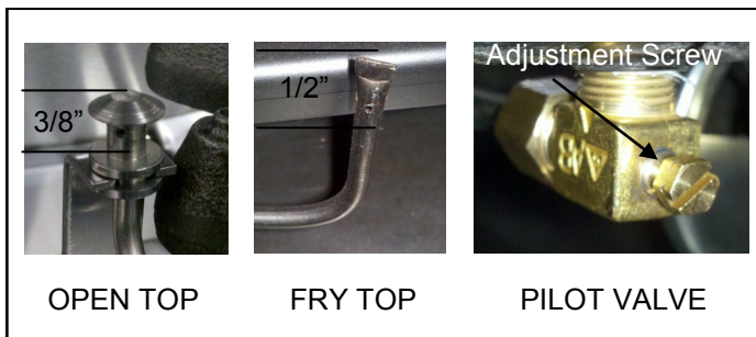
Figure 6. Pilot Flame
