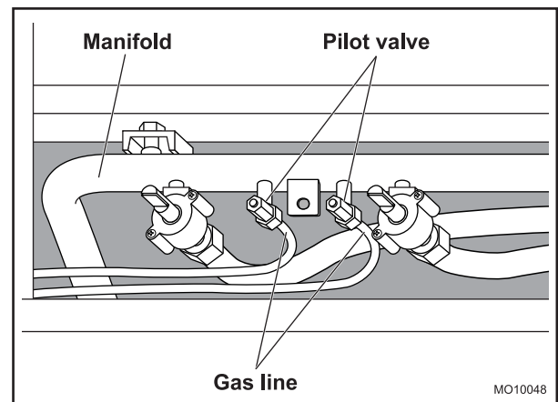
Figure 5. Pilot Valve
