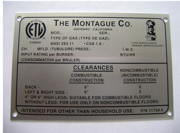
FIGURE1. TYPICAL I.D. PLATE
