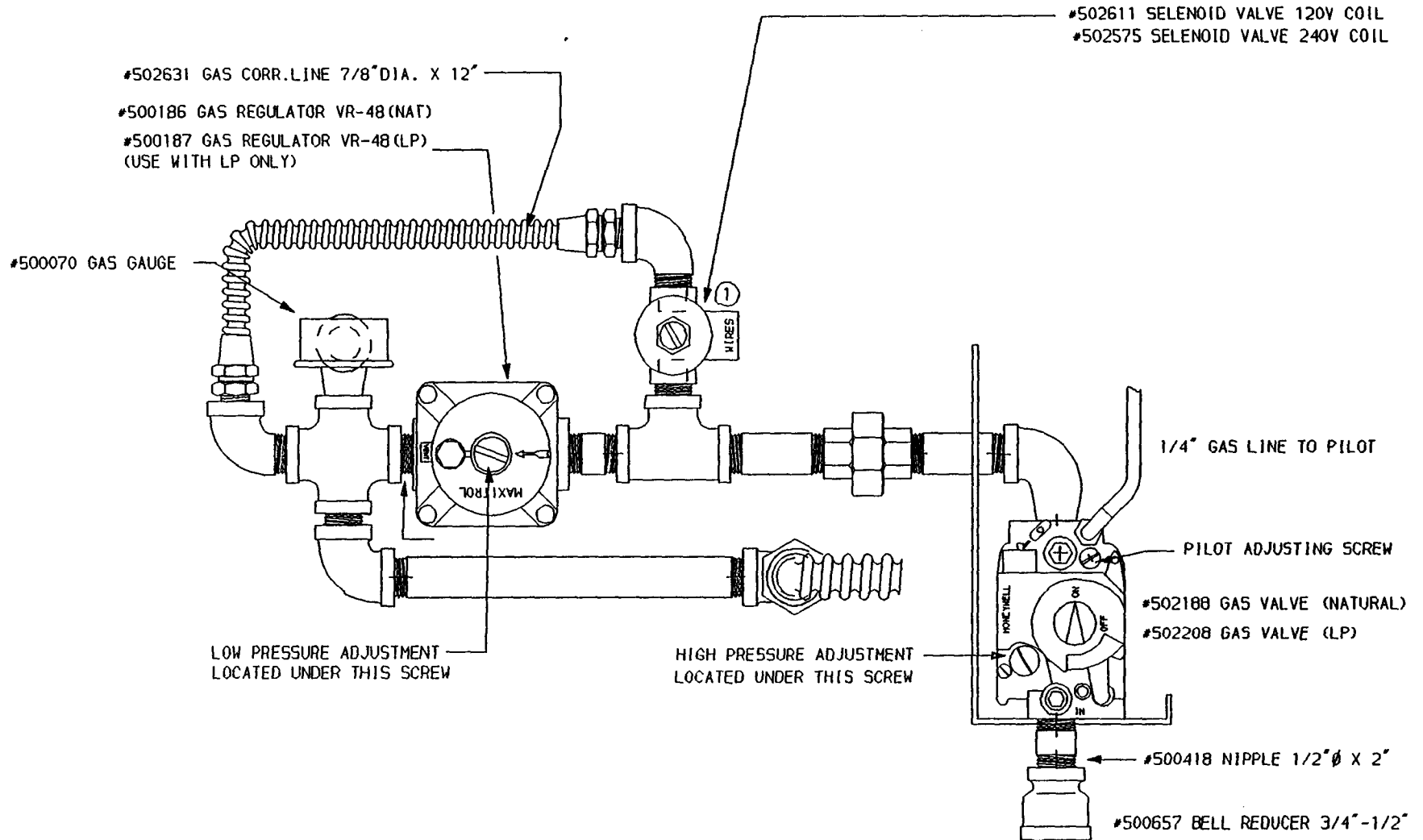
GAS DISTRIBUTION SYSTEM FIGURE 5
