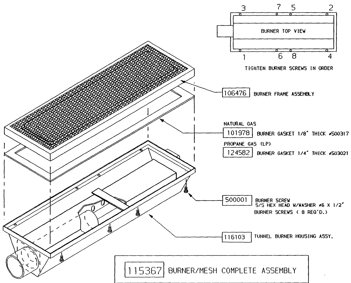
BURNER ASSEMBLY FIGURE 4
