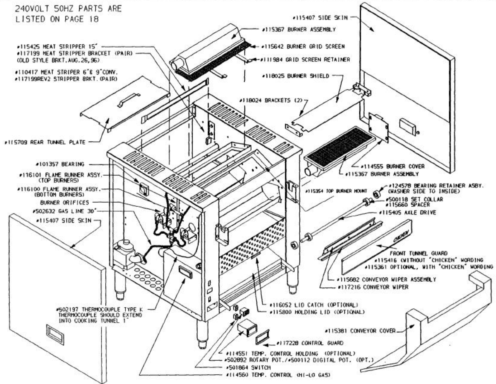
EXPLODED VIEW FIGURE 2
