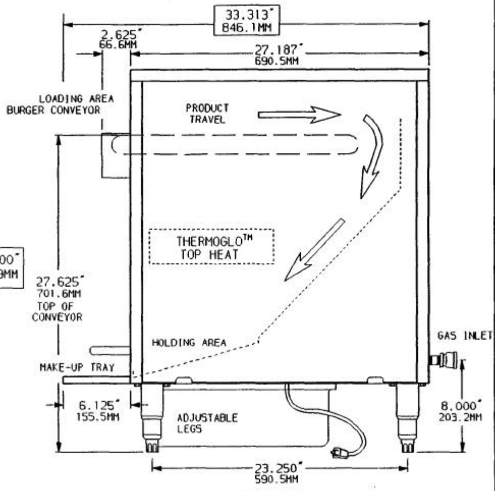
SIDE VIEW
