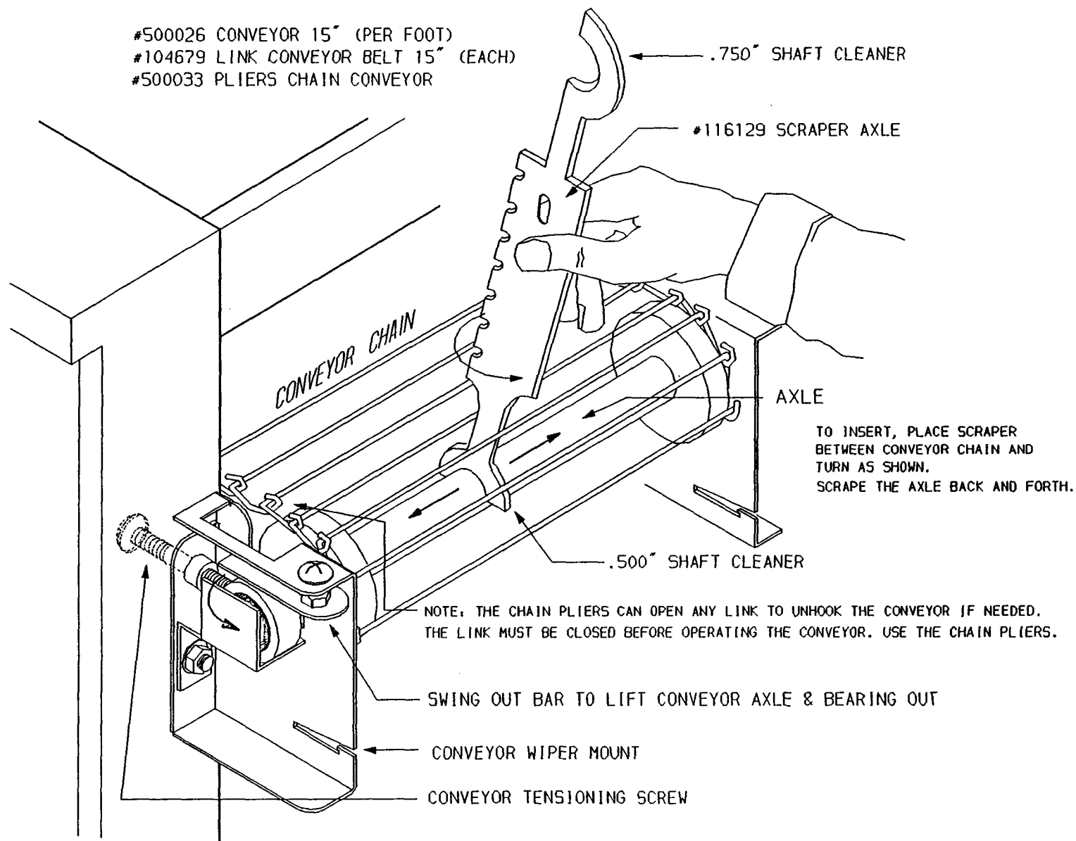
AXLE SCRAPER FIGURE 6
