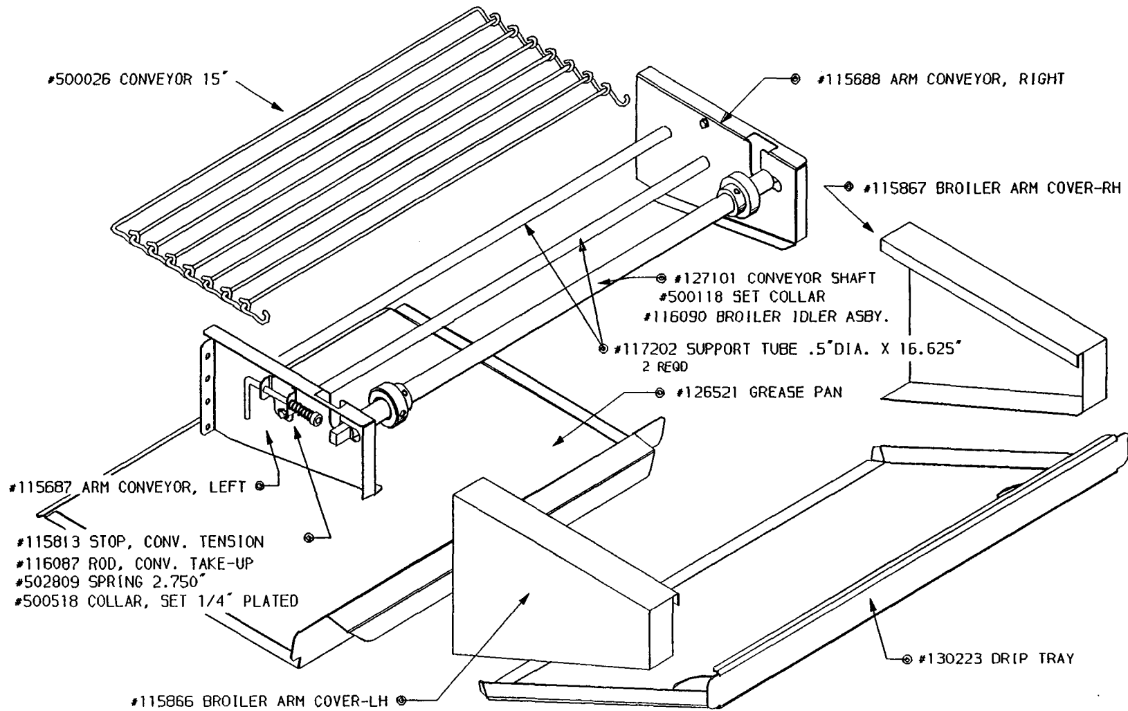
KIT, BROILER ARM EXTENSION 15" (OPTIONAL) (130224)
