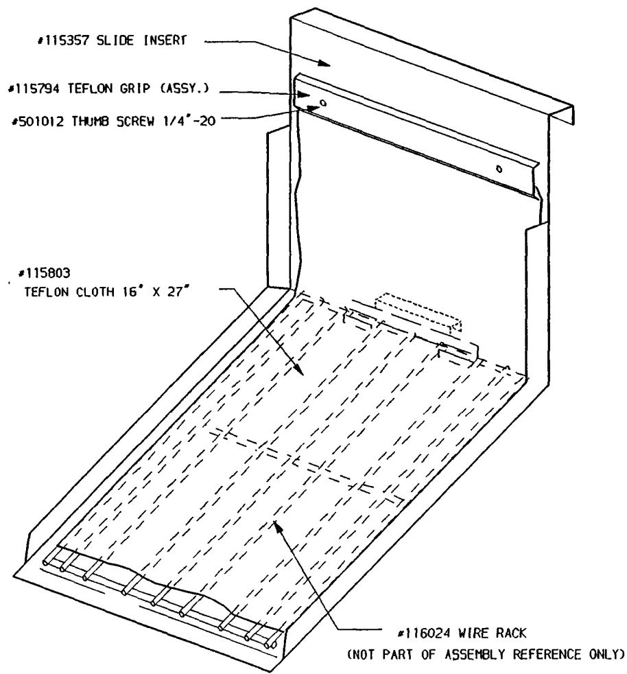
#115799 SLIDE ASSEMBLY
