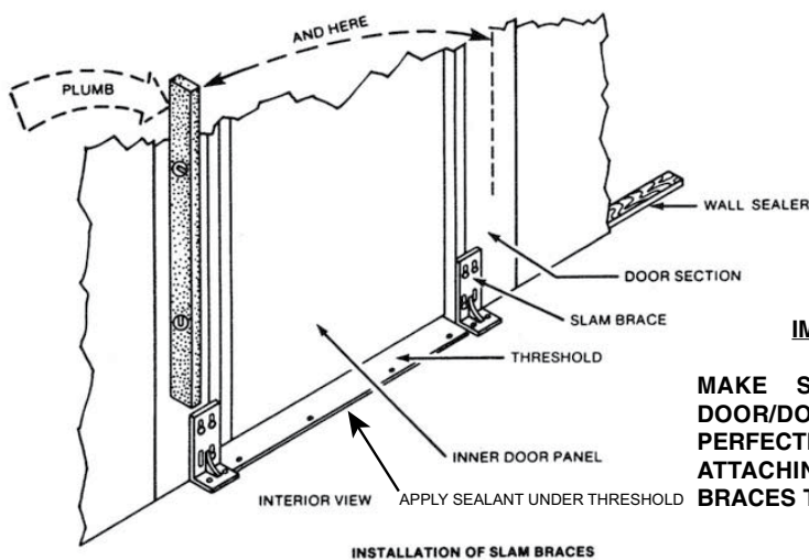
INSTALLATION OF SLAM BRACES
