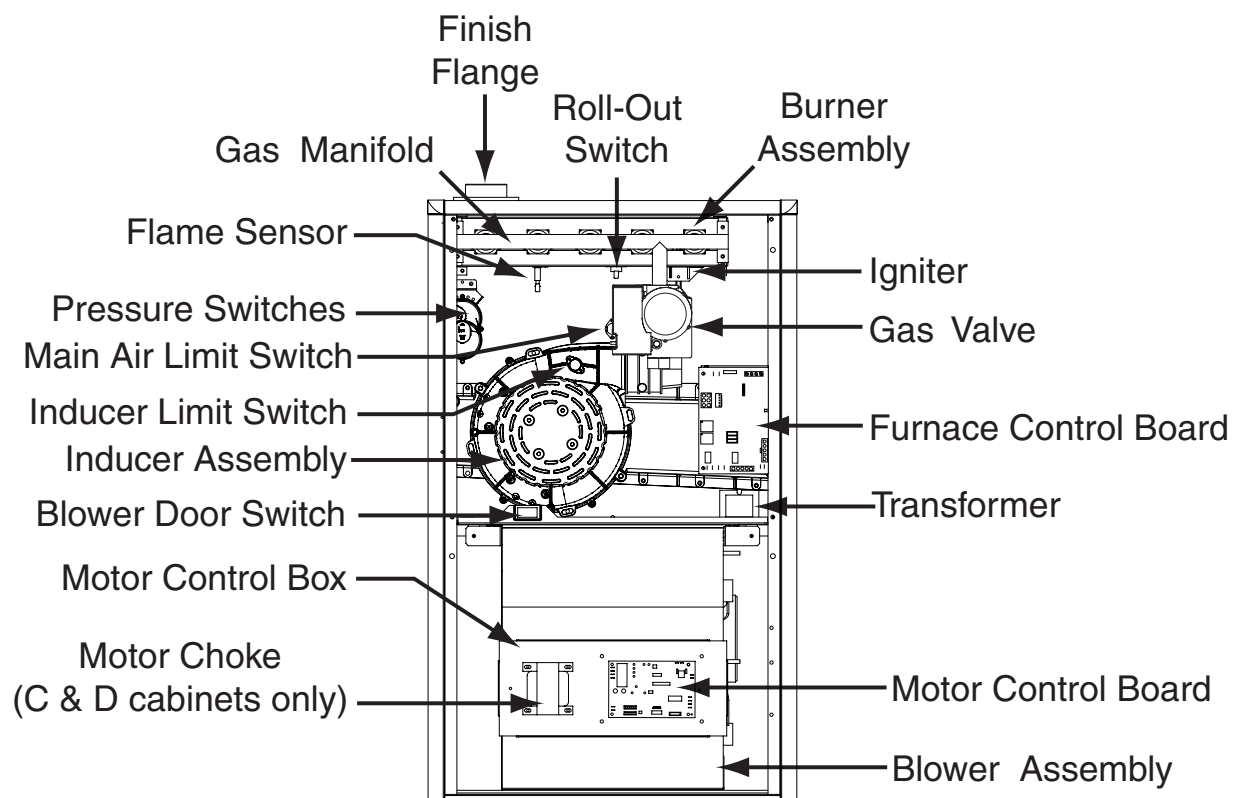
Figure 29. Component Locations
